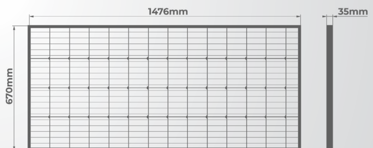
KT70729 DIMENSIONS
